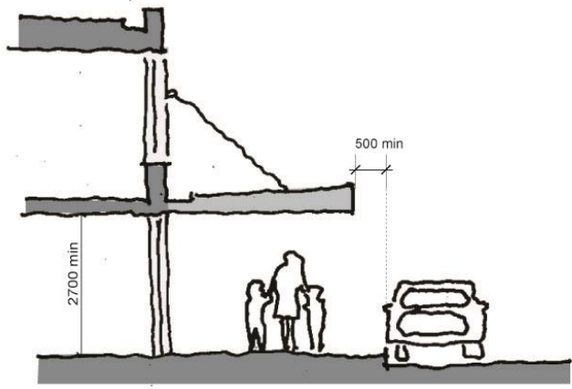
TYPICAL SECTION
