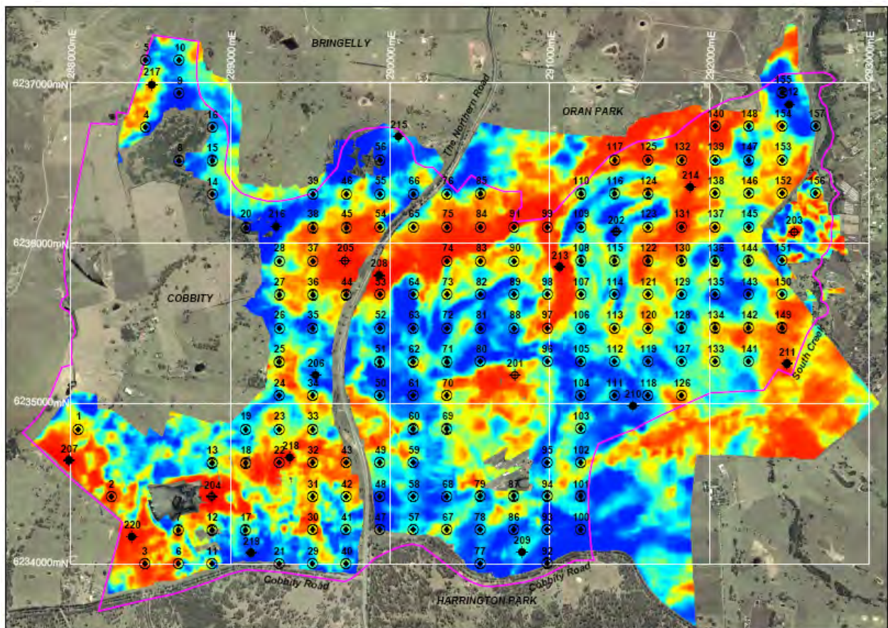
Apparent Conductivity (see Drawing 15, Appendix A)
