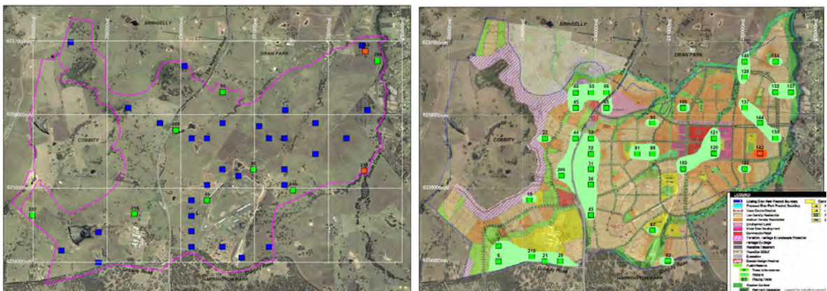
L & R: Aggressivity to concrete at 0.5m and 1.5 m depths (See Drawings 18 & 19, Appendix A)
