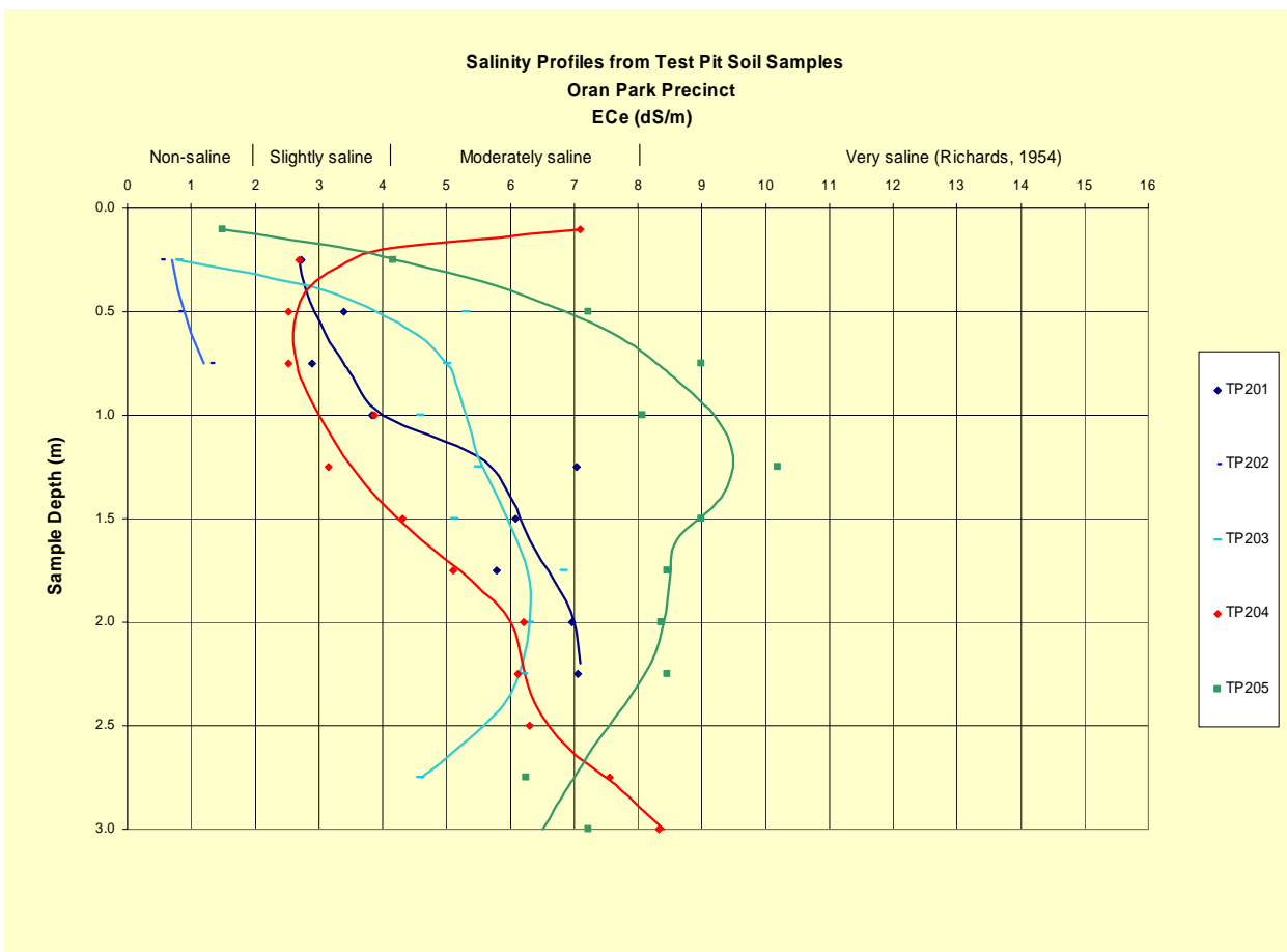
Figure 1 – Vertical Soil Salinity Profiles
