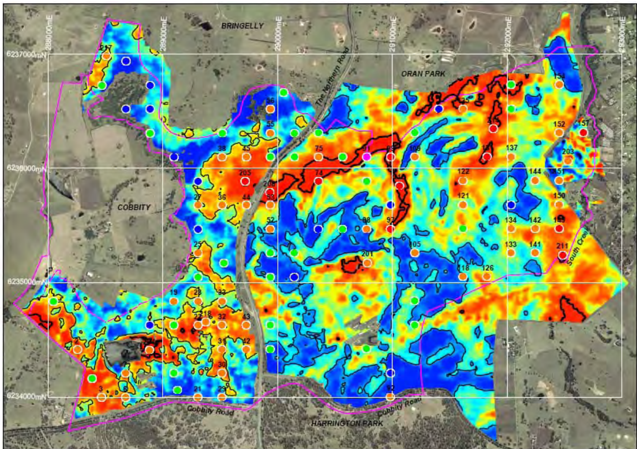
Apparent Salinity (see Drawing 16, Appendix A)
