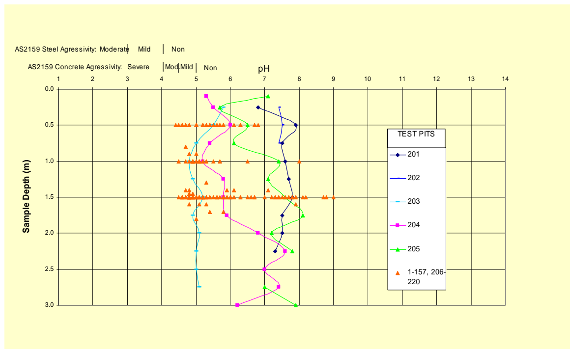
Figure 4 – pH Profiles, Oran Park Precinct
